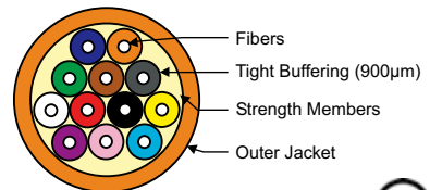
Distribution Cables
