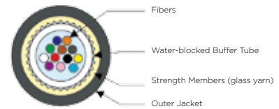
OSP Dielectric Single Loose Tube Cable
