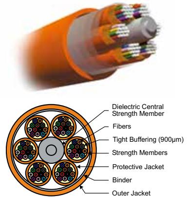
Multi-unit Distribution Cables
