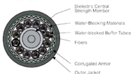
OSP Armored Stranded Loose Tube Cable
