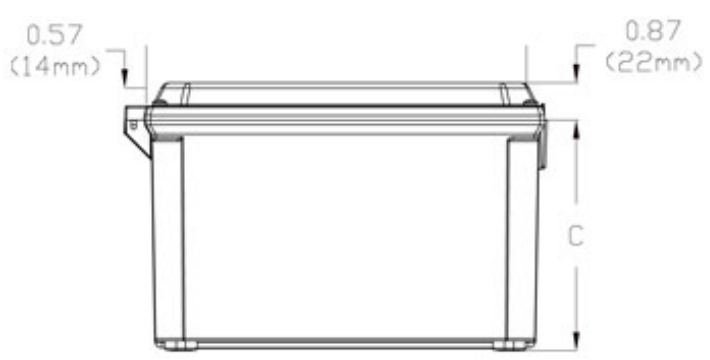
End View
