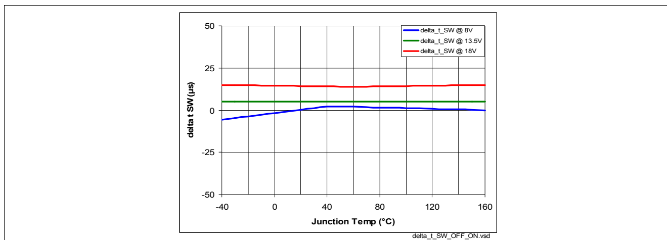
Figure 40 Turn ON / OFF matching \Delta t_{SW} = f(T_J; V_S) , R_L = 12 \Omega
