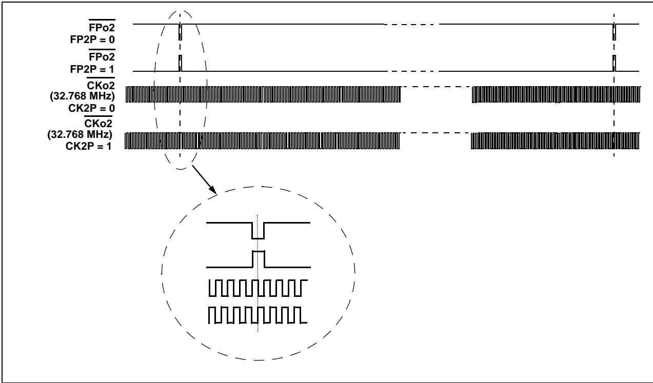
Figure 12 - \overline{\text{FPo2}} and \overline{\text{CKo2}} Output Timing when the \text{CKFP2} Bit = 0
