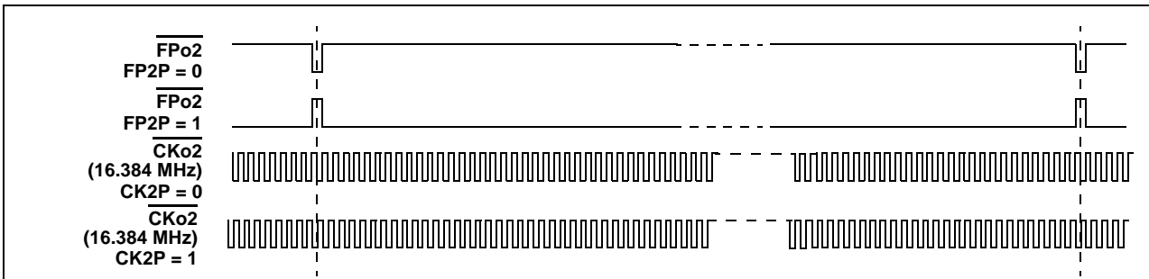
Figure 13 - \overline{\text{FPo2}} and \overline{\text{CKo2}} Output Timing when the \text{CKFP2} Bit = 1
