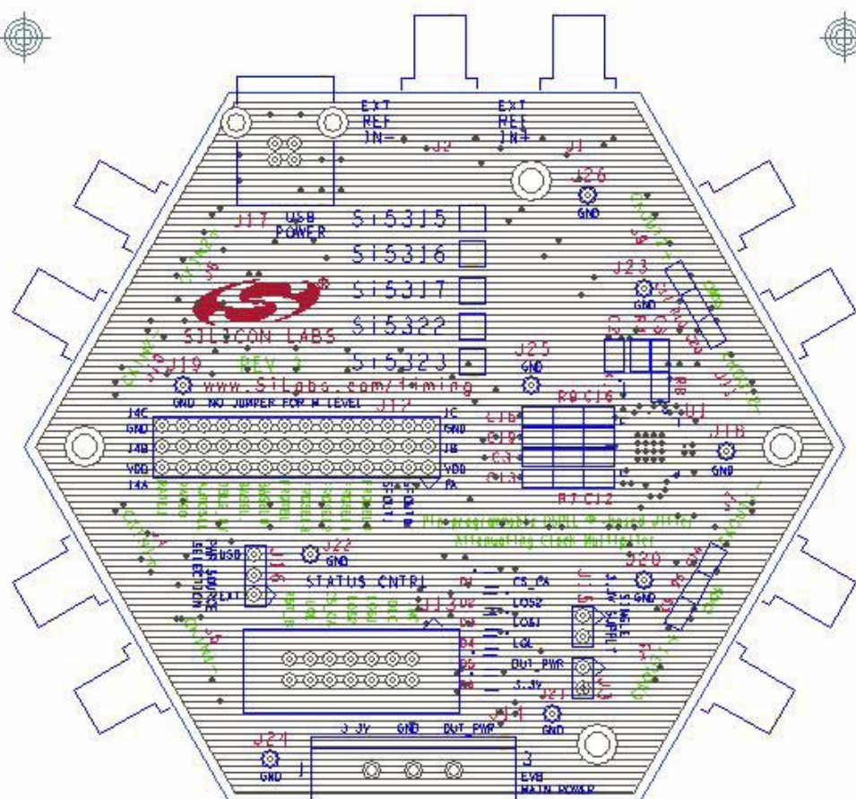
Figure 10. Layer 5, FILTER_DUT_PWR
