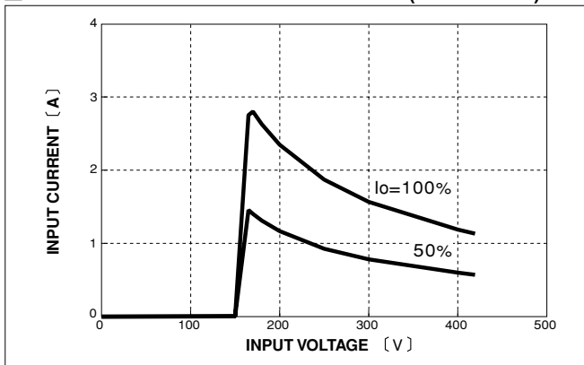
INPUT CURRENT CHARACTERISTICS (DBS400B12)
