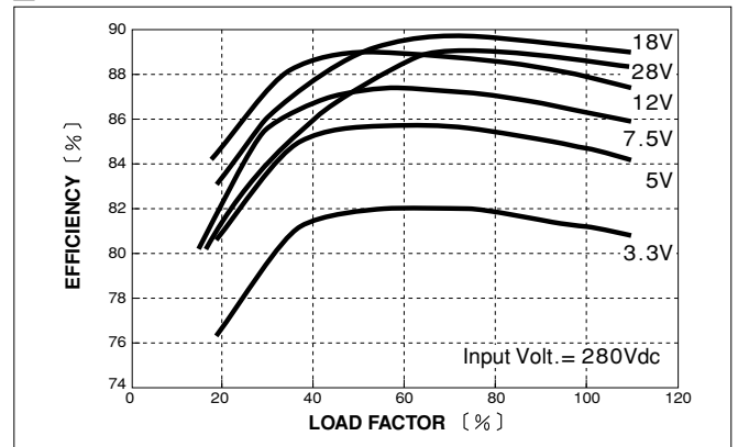
EFFICIENCY CHARACTERISTICS
