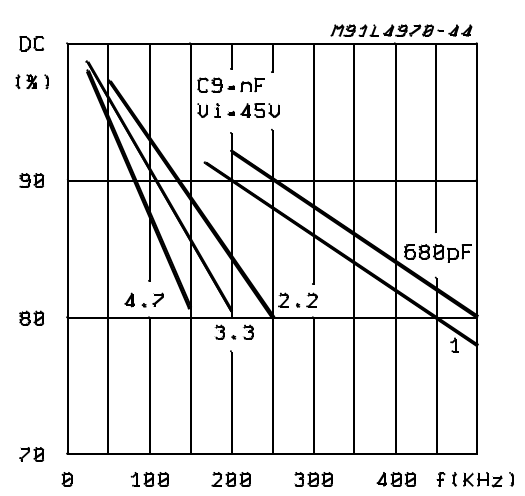
Figure 19: Max. Duty Cycle vs. Frequency
