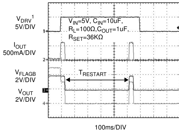
Figure 17. T_{RESTART} Response
