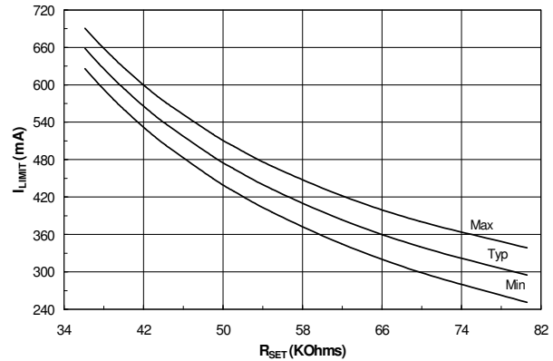
Figure 23. I LIM vs R SET
