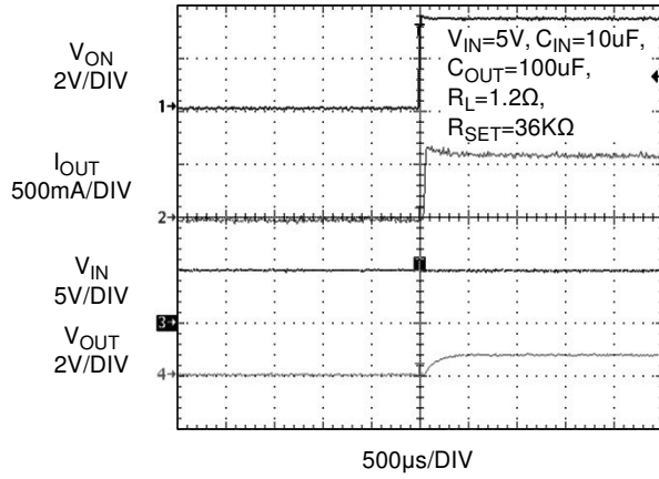
Figure 19. Current Limit Response (Output is loaded with 1.2 \Omega resistor and C_{OUT}=100\mu F)
