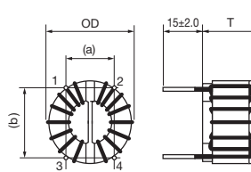
● SC Coils horizontal type (10A-)
