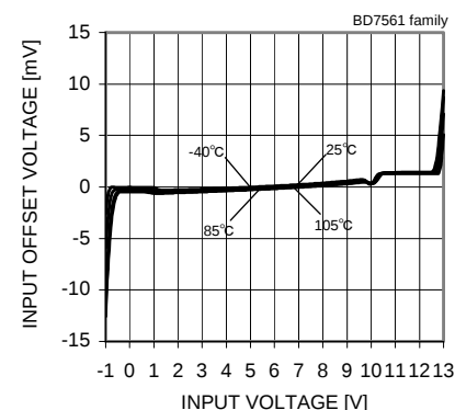
Fig. 15 Input Offset Voltage – Input Voltage ( V_{DD}=12[V] )
