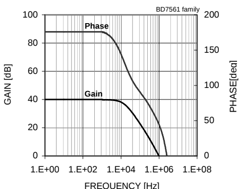
Fig. 23 Gain - Frequency
