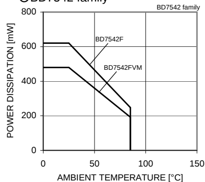
Fig. 70 Derating Curve
