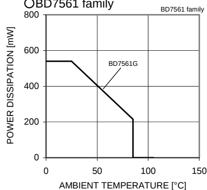
Fig. 1 Derating Curve
