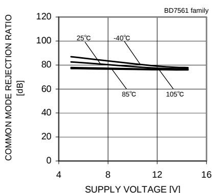
Fig. 18 Common Mode Rejection Ratio – Supply Voltage ( V_{DD}=12[V] )
