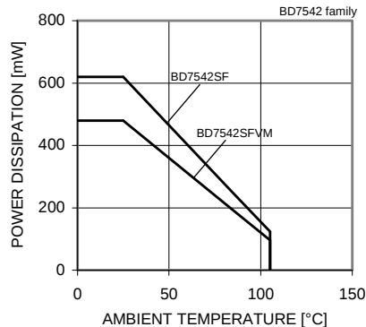
Fig. 71 Derating Curve
