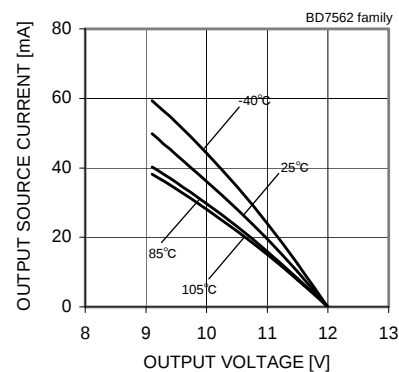
Fig. 32 Output Source Current – Output Voltage (VDD=12[V])
