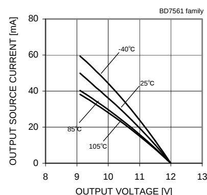
Fig. 9 Output Source Current – Output Voltage ( V_{DD}=12[V] )
