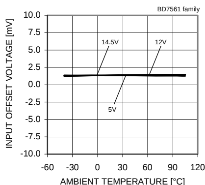
Fig. 14 Input Offset Voltage – Ambient Temperature ( V_{icm}=V_{DD} , V_{OUT}=V_{DD}/2 )
