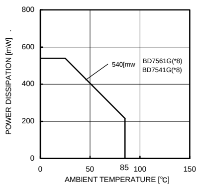
(c) BD7561G
