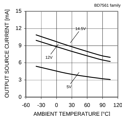
Fig. 10 Output Source Current – Ambient Temperature( V_{OUT}=V_{DD}-0.4[V] ) (*) The above data is ability value of sample, it is not guaranteed. BD7561 : -40[°C]~+85[°C] BD7561S : -40[°C]~+105[°C]
