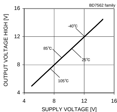
Fig. 28 Output Voltage High – Supply Voltage (RL=10[kΩ])
