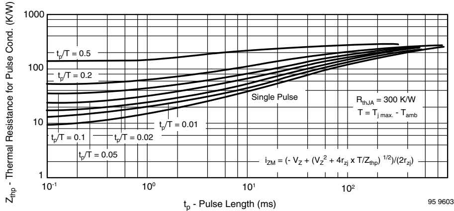
Fig. 10 - Thermal Response
