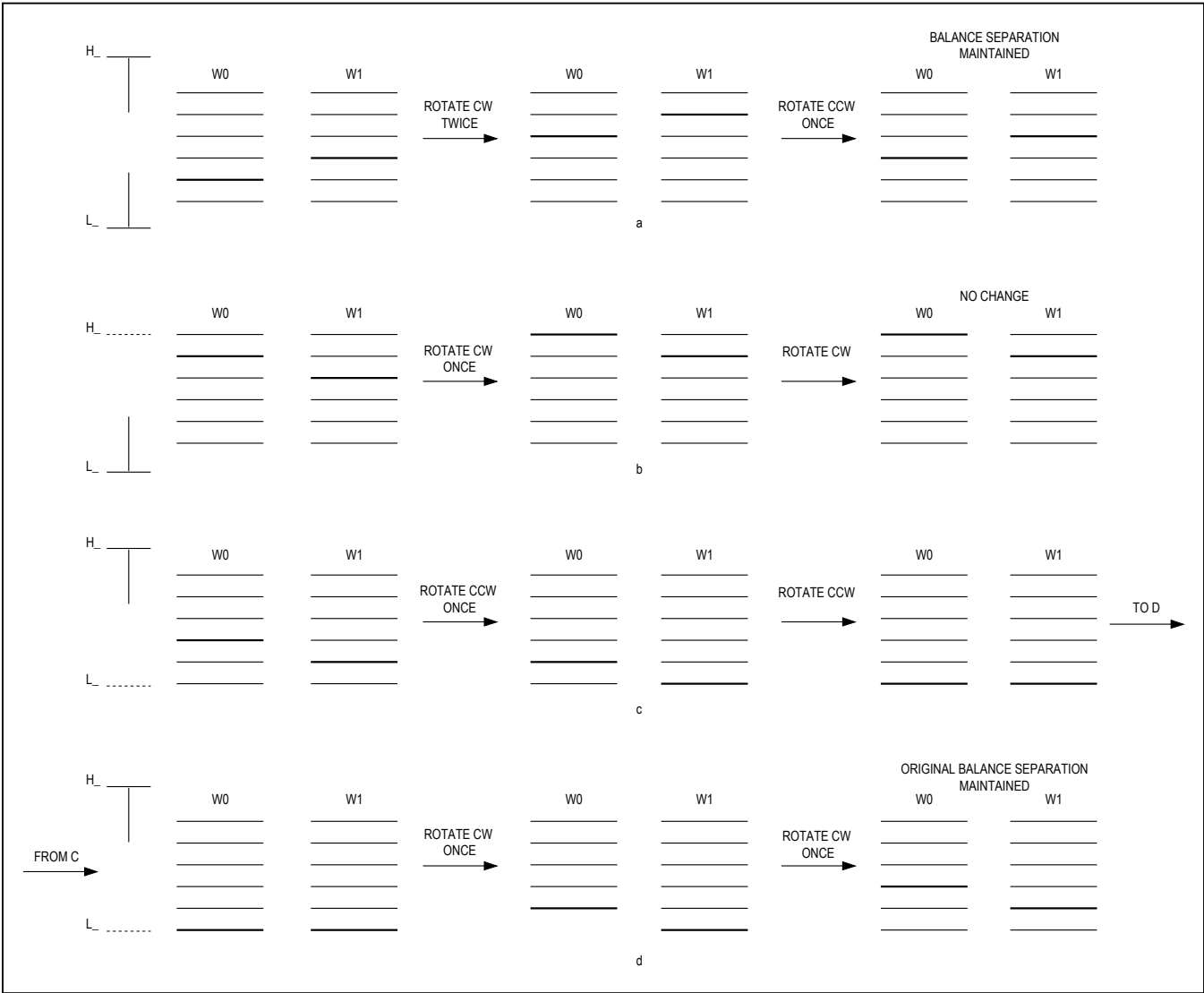
Figure 2. Volume-Control Operation
