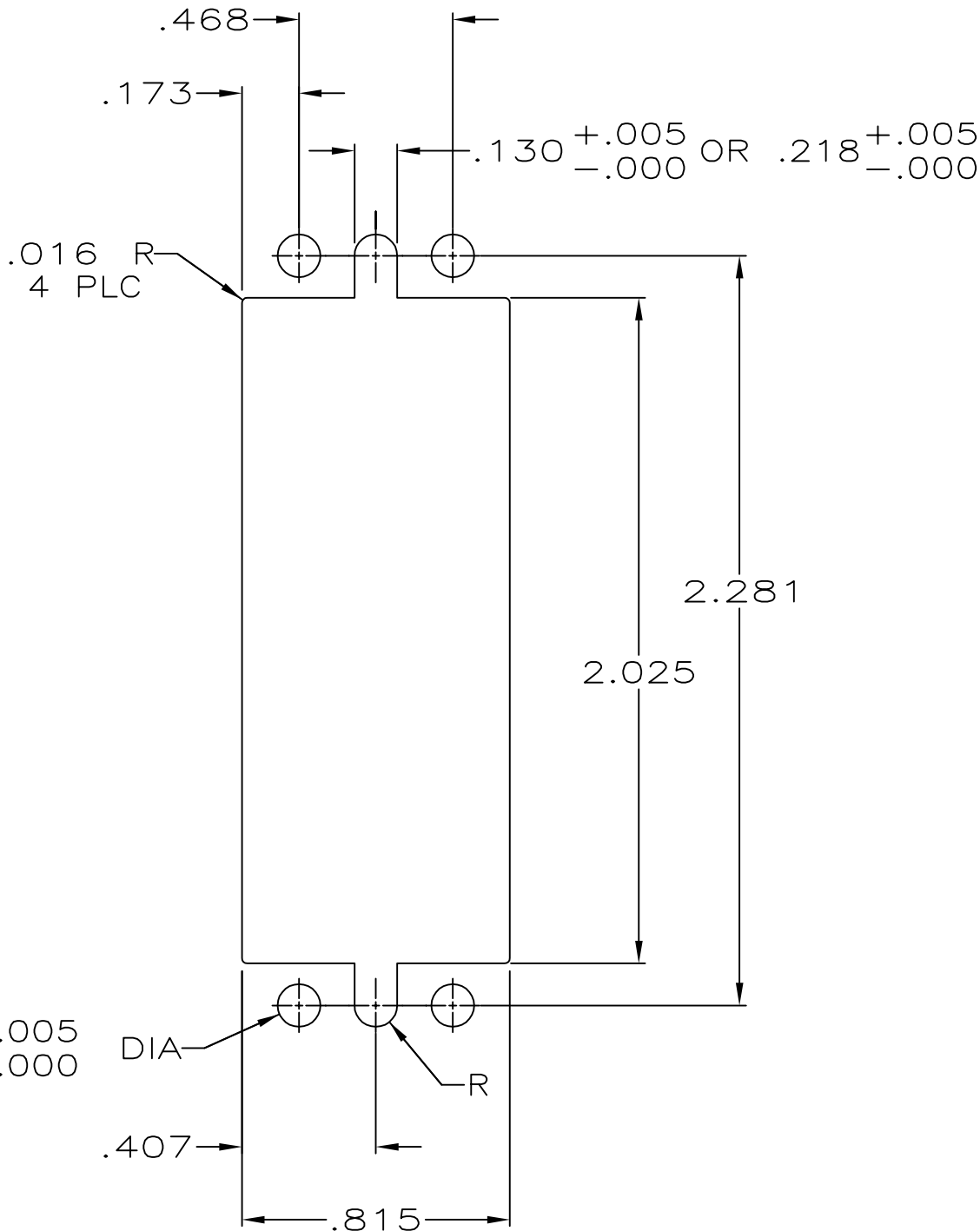
SUGGESTED PANEL CUTOUT
