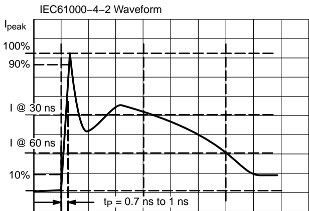
Figure 8. IEC61000-4-2 Spec
