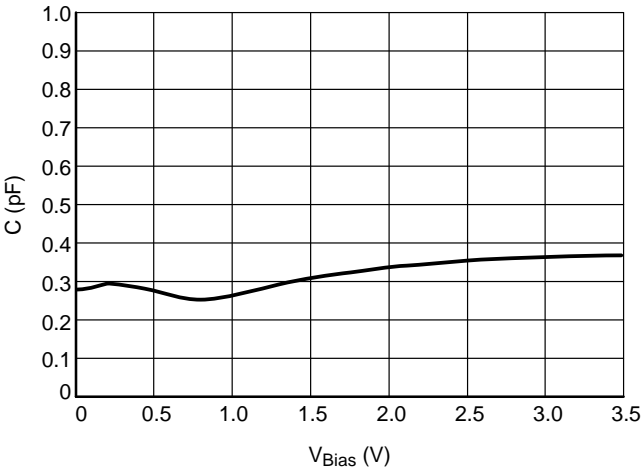
Figure 1. CV Characteristics
