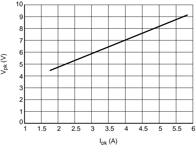
Figure 2. Clamping Voltage vs Peak Pulse Current ( t p = 8/20 μs)
