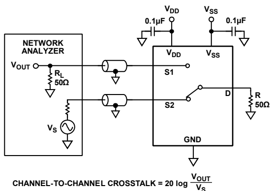
Figure 21. Channel-to-Channel Crosstalk
