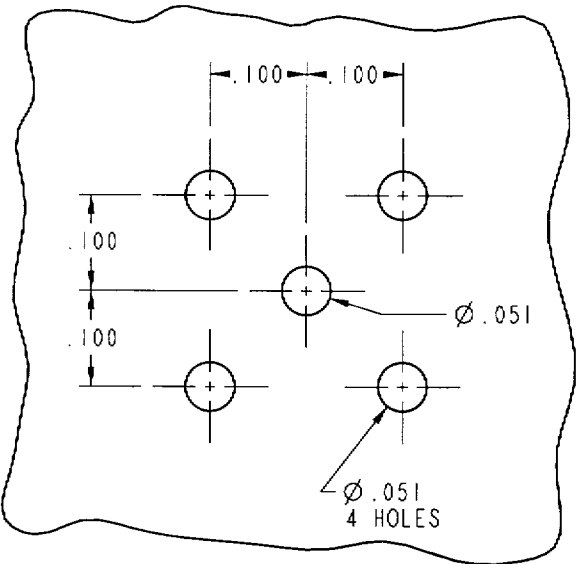
MOUNTING HOLE DIMENSIONS SCALE 5.000
