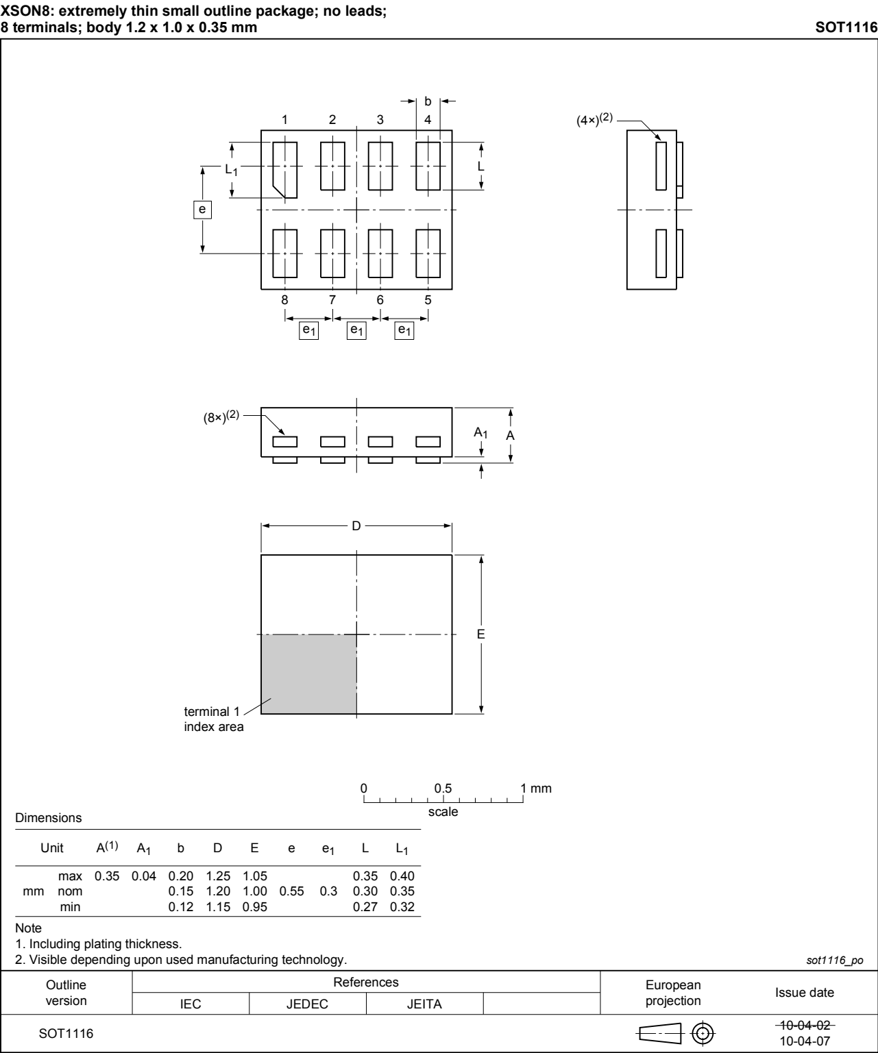
Figure 13. Package outline SOT1116 (XSON8)
