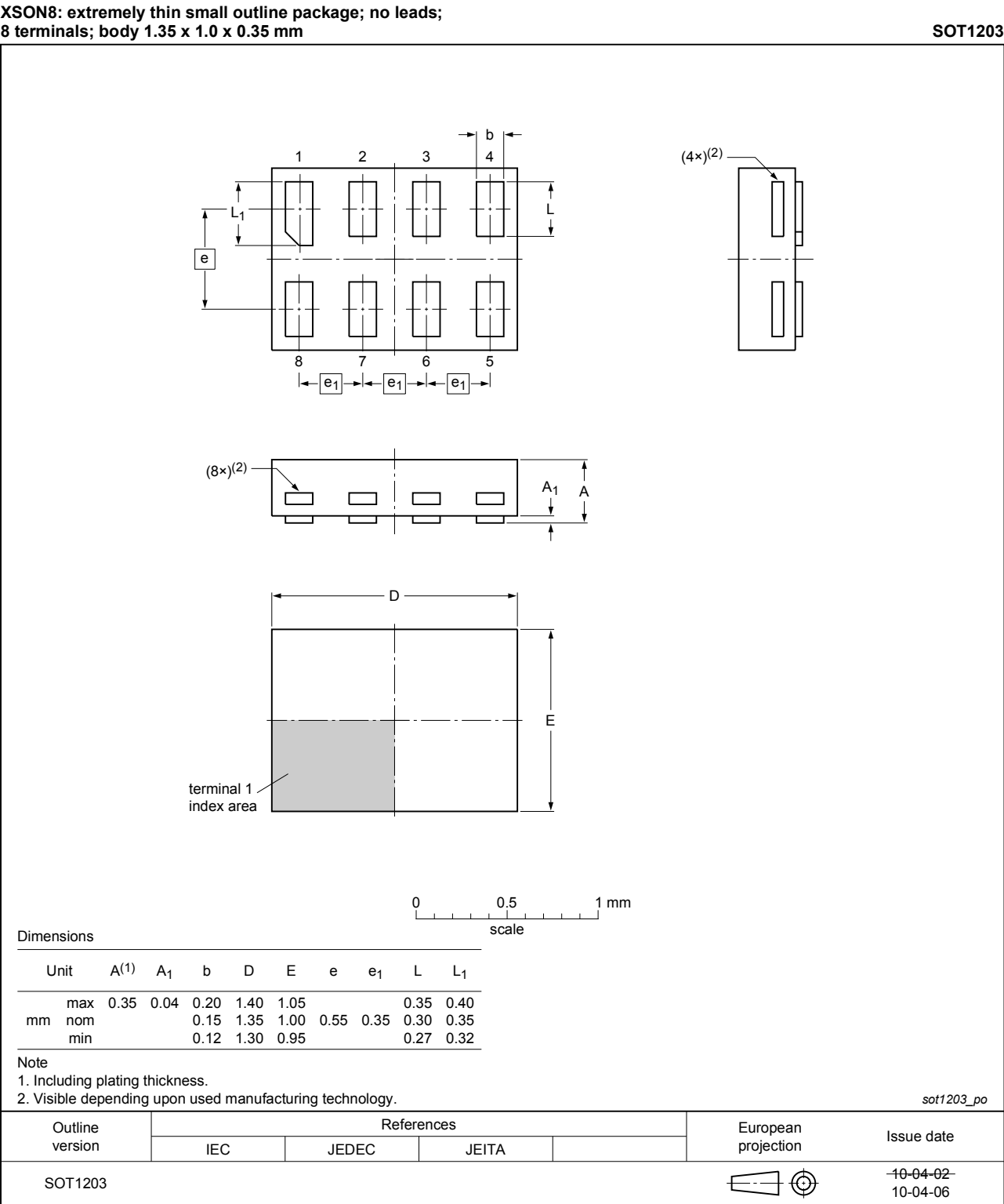
Figure 14. Package outline SOT1203 (XSON8)
