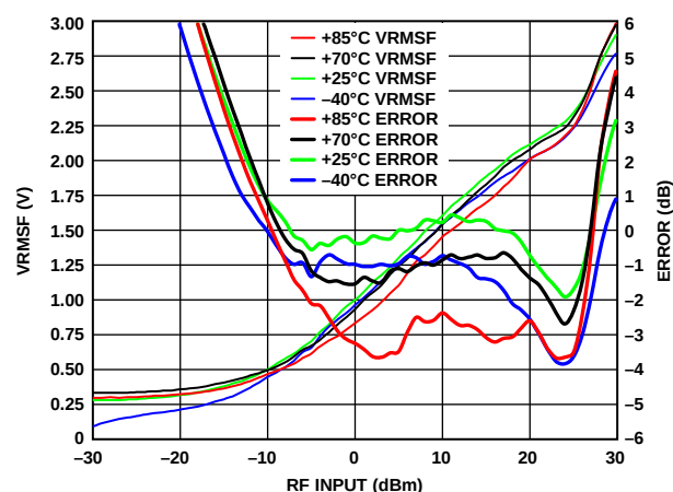
Figure 20. VRMSF and Error vs. RF Input and Temperature at 7 GHz, Error Calculated Using Linear Regression of Data Between 20 dBm and 0 dBm, TADJS = 0.8 V, TADJI = 0.2 V, CHPF+/CHPF- Open
