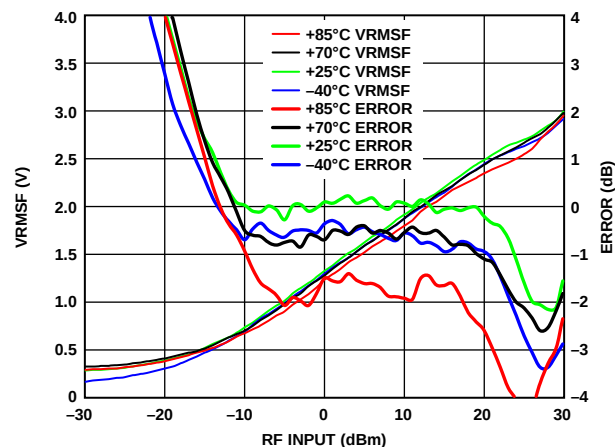
Figure 18. VRMSF and Error vs. RF Input Level and Temperature at 5 GHz, Error Calculated Using Linear Regression of Data Between 15 dBm and -10 dBm, TADJS = 0.2 V, TADJI = 0.2 V, CHPF+/CHPF- Open
