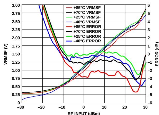
Figure 19. VRMSF and Error vs. RF Input Level and Temperature at 6 GHz, Error Calculated Using Linear Regression of Data Between 20 dBm and -5 dBm, TADJS = 0 V, TADJI = 0.2 V, CHPF+/CHPF- Open
