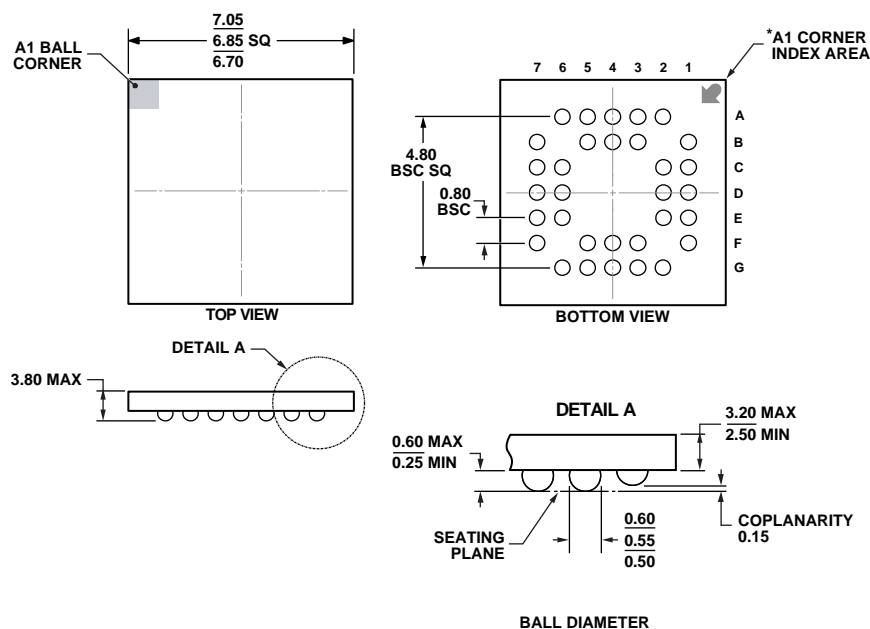
Figure 24. 32-Lead Ceramic Ball Grid Array [CBGA] (BG-32-3) Dimensions shown in millimeters
