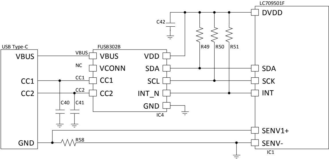
Figure 29: Firmware: FW05 Parts example around Port control IC
