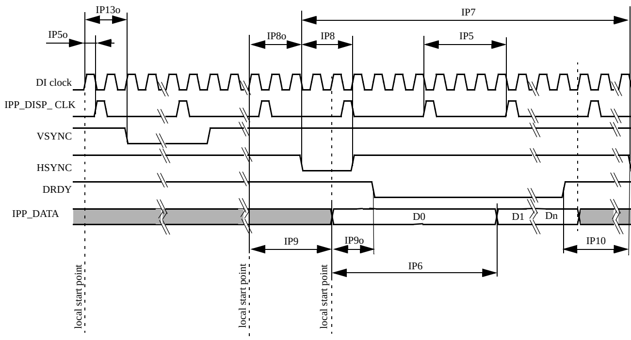
Figure 68. TFT Panels Timing Diagram—Horizontal Sync Pulse
