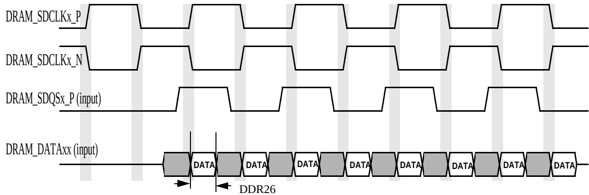
Figure 25. DDR3/DDR3L Read Cycle
