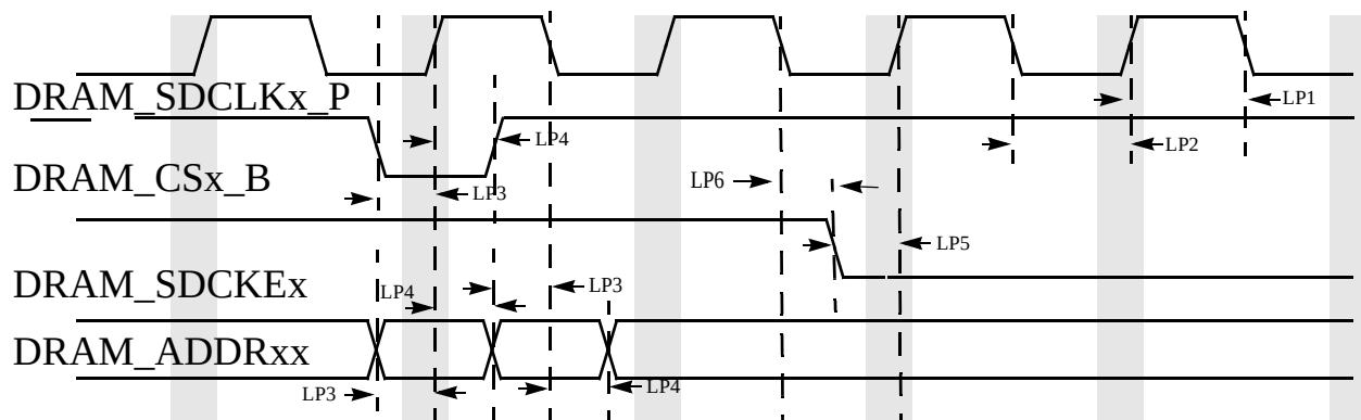
Figure 26. LPDDR2 Command and Address Timing Parameters
