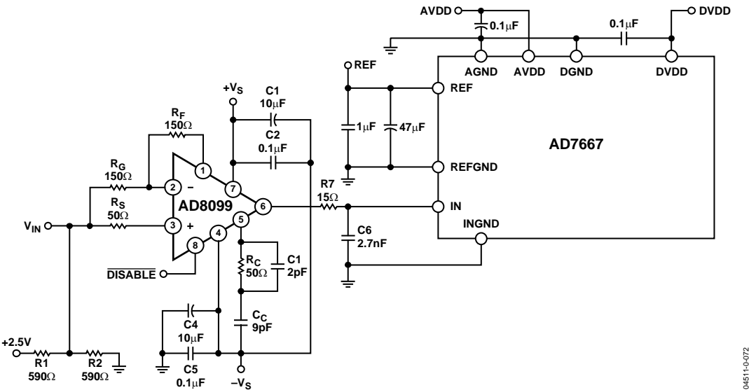
Figure 76. ADC Driver
