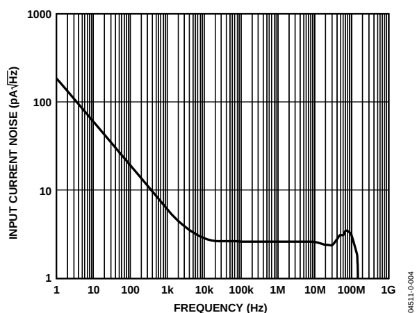
Figure 48. Input Current Noise vs. Frequency ( \overline{\text{DISABLE}} = \text{Open} )
