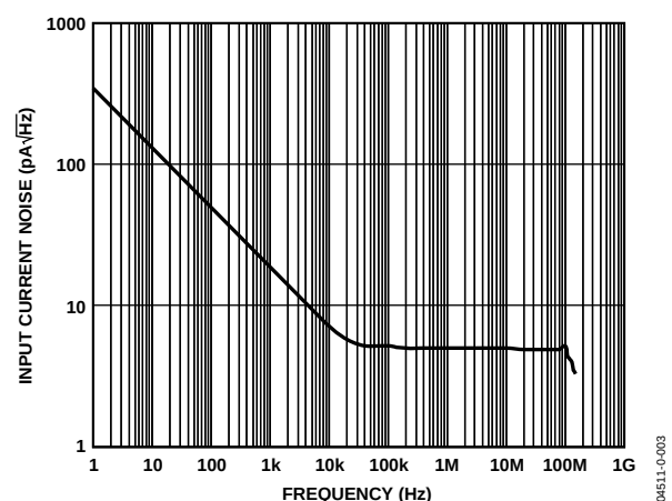
Figure 51. Input Current Noise vs. Frequency ( \overline{\text{DISABLE}} = +V_S )
