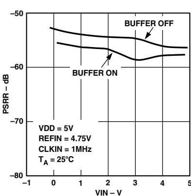
TPC 5. PSRR vs. VIN (Buffered and Unbuffered)
