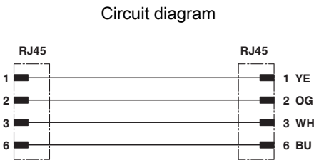
Contact assignment of RJ45 plugs
