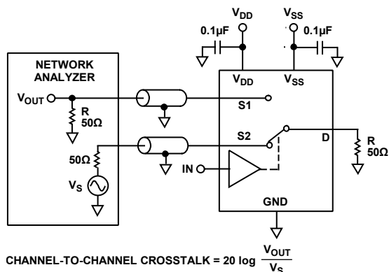
Figure 23. Channel-to-Channel Crosstalk
