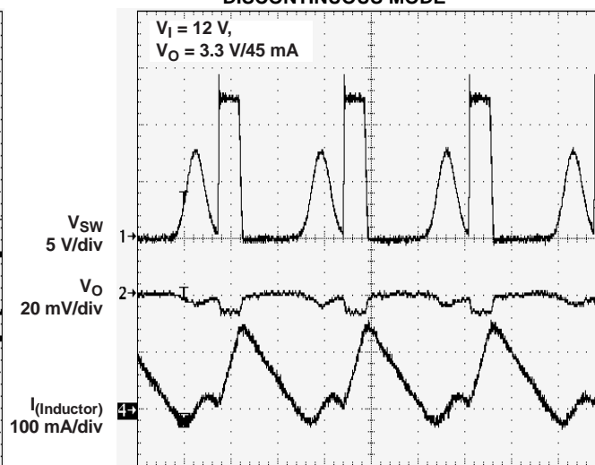
500 ns/div Figure 10.
