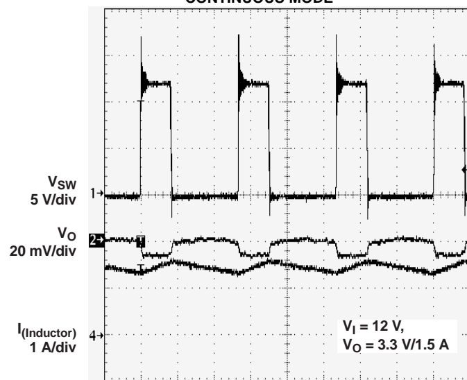
500 ns/div Figure 9.
