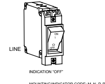
MARKING DETAIL "B" (SEE TABLE)
