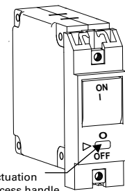
Actuation access handle (see note)
