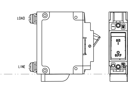
1-POLE (CF1, CG1,C11,C21) w/ ARC CHUTE (NO BARRIER)
