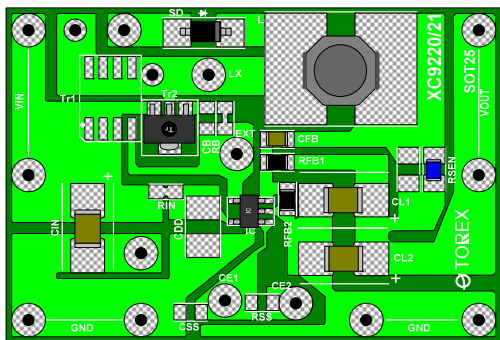
[Board layout when XC9220/XC9221 series is mounted with external components]
