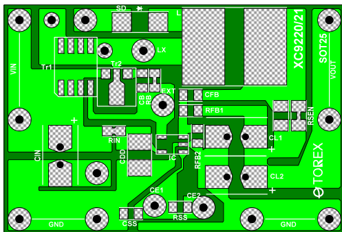
[PC board for the XC9220/XC9221 series]
