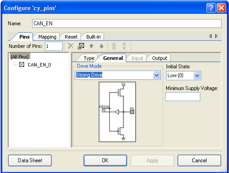
Figure 5-24. CAN_EN Configuration: Pins > General Tab
