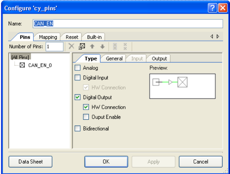
Figure 5-23. CAN_EN Configuration: Pins > Type Tab
