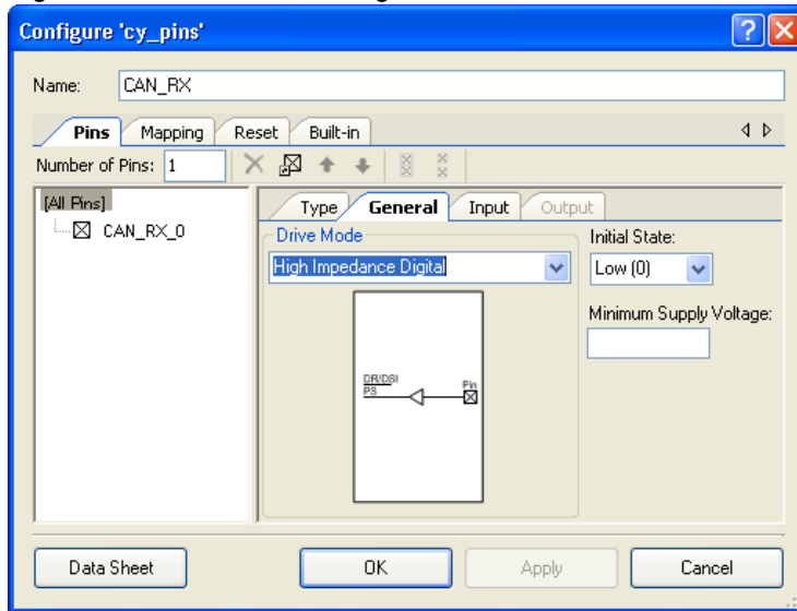
Figure 5-21. CAN_RX Configuration: Pins &gt; General Tab
