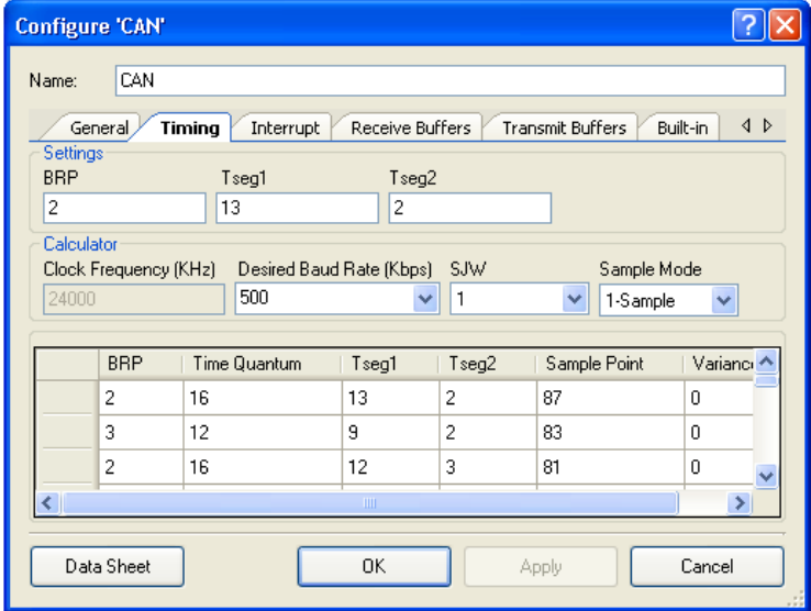
Figure 5-5. CAN Configuration: Timing Tab
