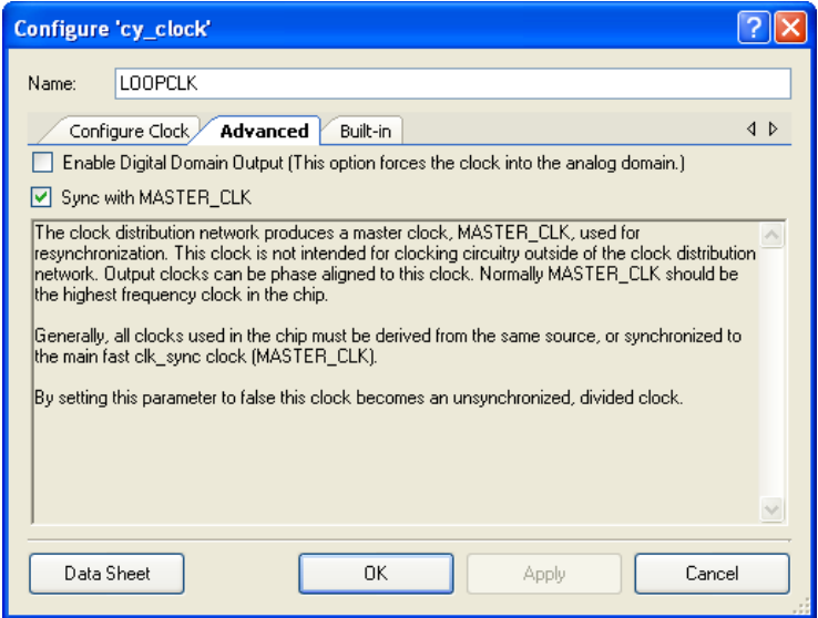
Figure 5-16. LOOPCLK Configuration: Advanced Tab
