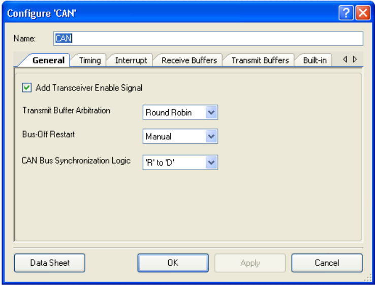
Figure 5-4. CAN Configuration: General Tab
