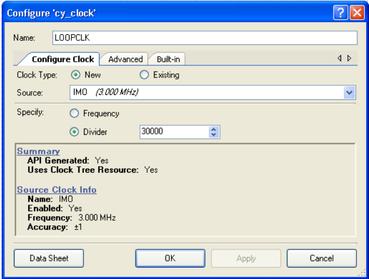
Figure 5-15. LOOPCLK Configuration: Configure Clock Tab
