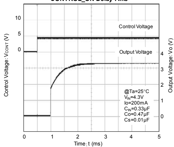
NJM12856_3.3V CONTROL_ON Delay Time
