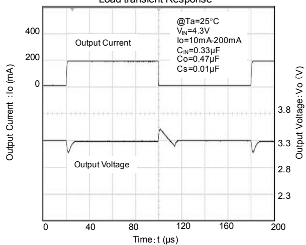
NJM12856_3.3V Load transient Response
