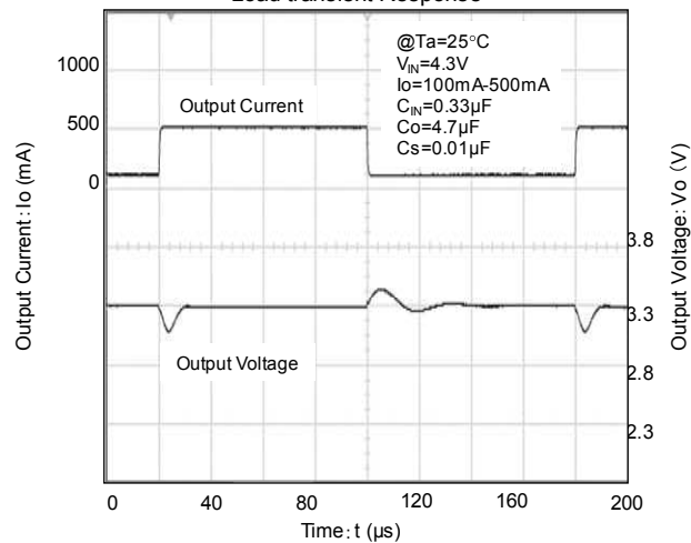
NJM12856_3.3V Load transient Response
