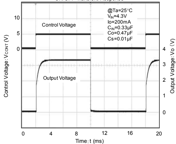
NJM12856_3.3V ON/OFF Transient Response
