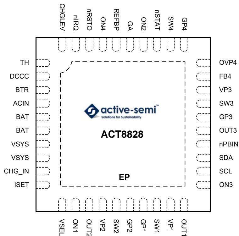
Thin - QFN (TQFN55-40)
