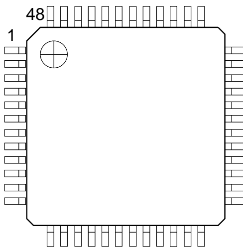
Figure 5: Pin Configuration, LQFP-48.
