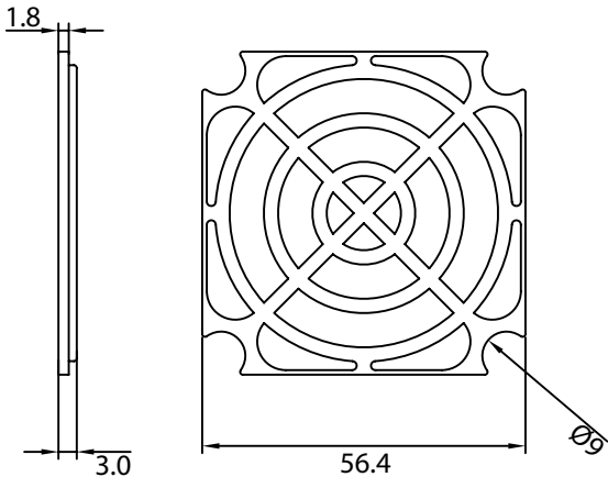
RETAINER
