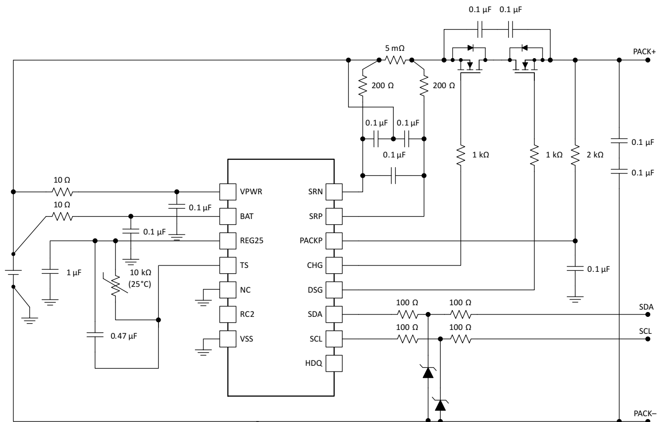
Figure 17. I²C Mode Schematic
