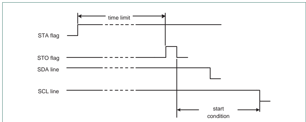
Fig 163. Forced access to a busy I2C-bus
