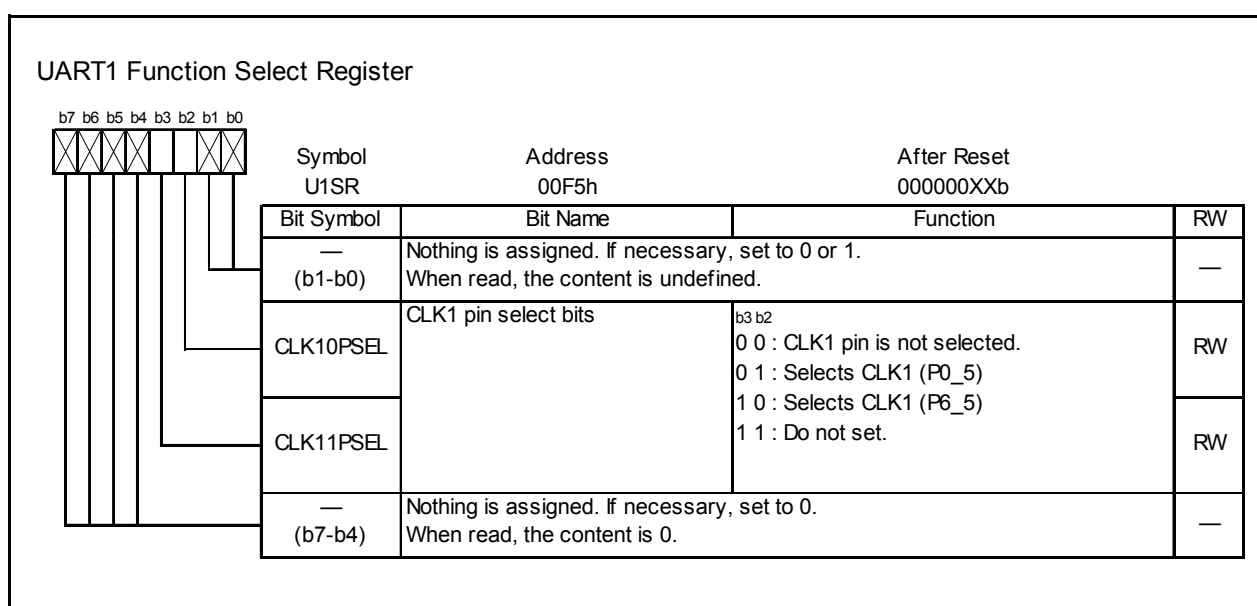
Figure 15.7 U1SR Register
