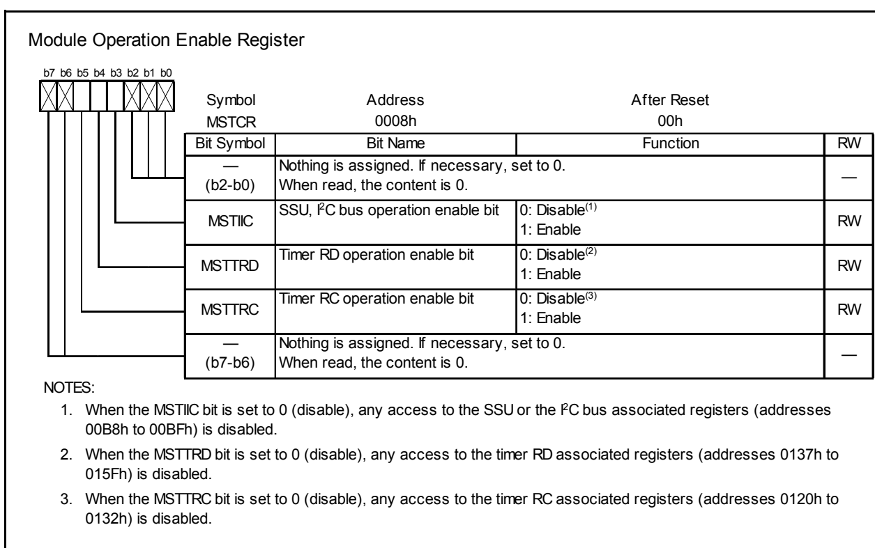
Figure 14.27 MSTCR Register
