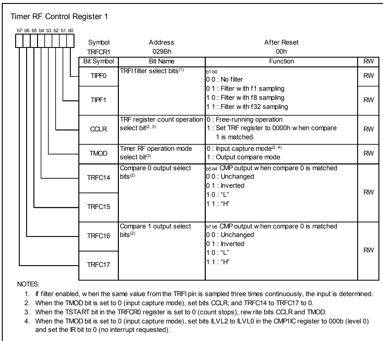
Figure 14.179 TRFCR1 Register
