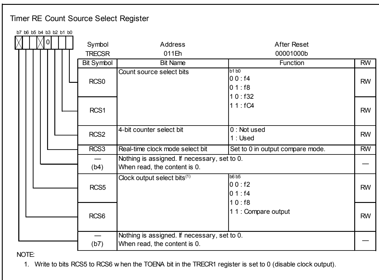
Figure 14.171 TRECSR Register in Output Compare Mode
