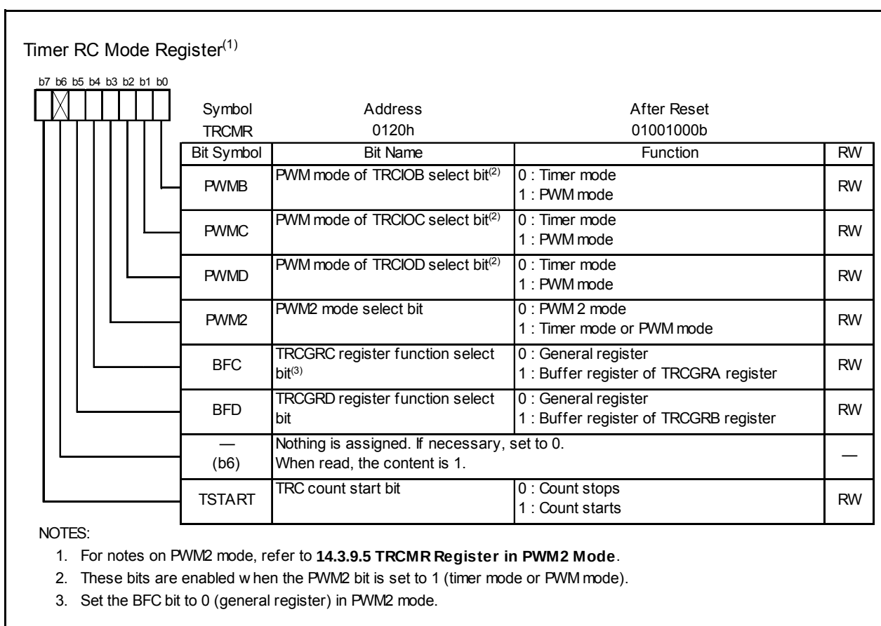
Figure 14.28 TRCMR Register
