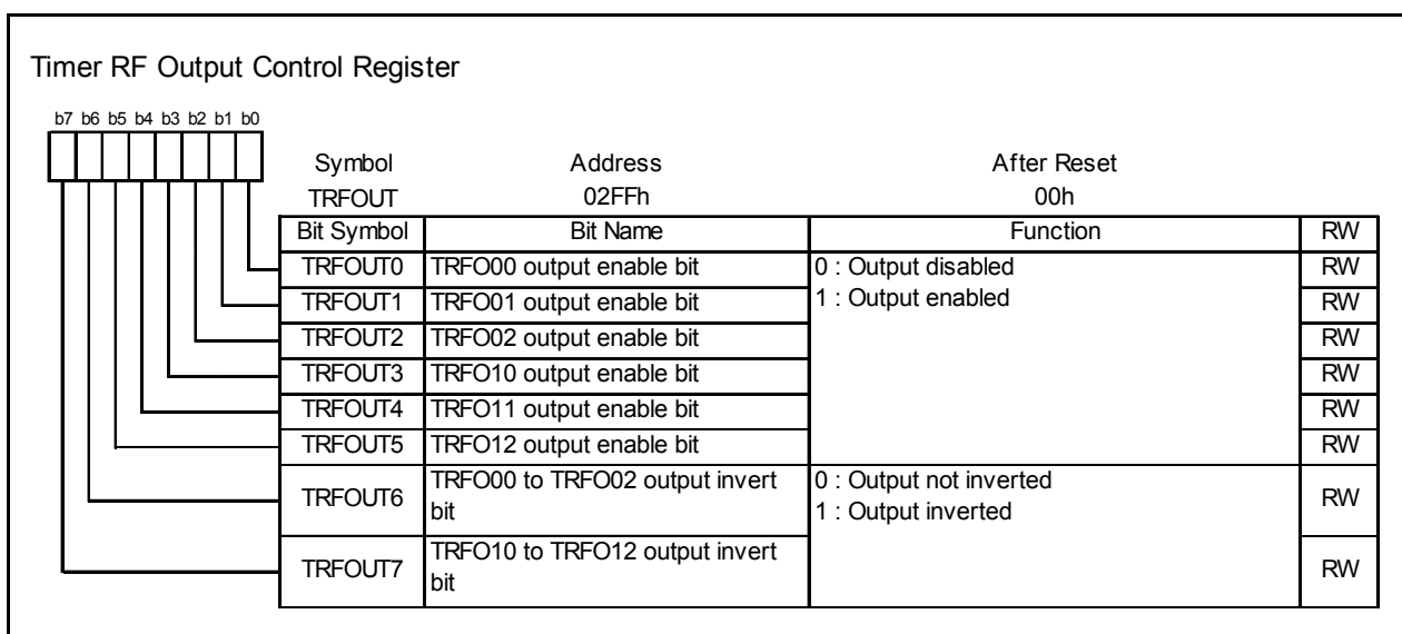
Figure 14.180 TRFOUT Register
