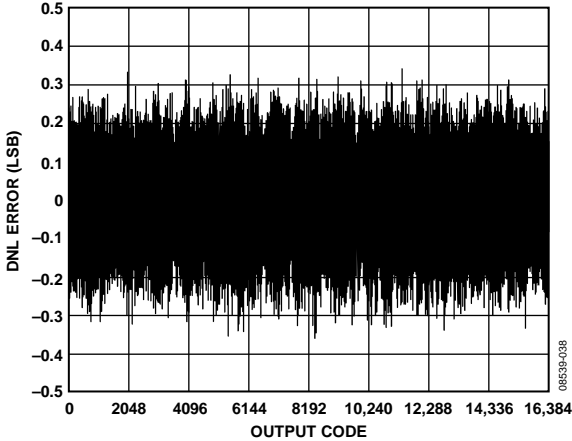
Figure 12. AD9649-80 DNL Error with f_{IN} = 9.7 MHz
