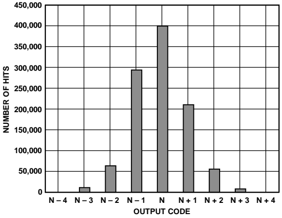
Figure 14. AD9649-80 Grounded Input Histogram
