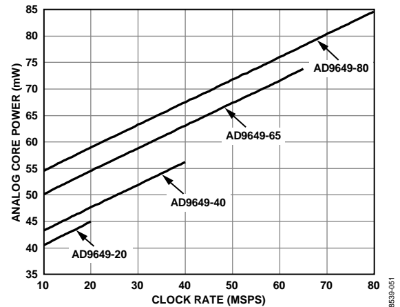
Figure 54. Analog Core Power vs. Clock Rate
