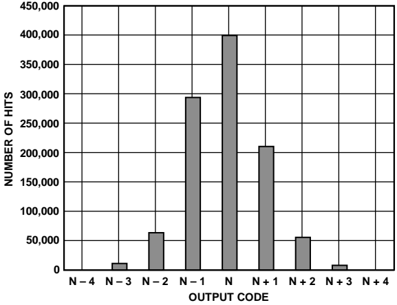
Figure 14. AD9649-80 Grounded Input Histogram
