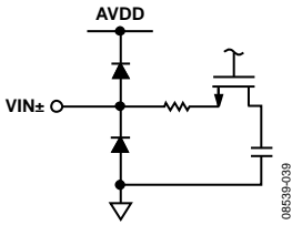
Figure 27. Equivalent Analog Input Circuit
