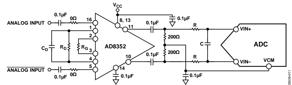
Figure 42. Differential Input Configuration Using the AD8352
