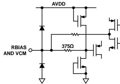
Figure 34. Equivalent RBIAS, VCM Circuit
