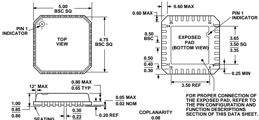
Figure 56. 32-Lead Lead Frame Chip Scale Package [LFCSP_VQ] 5 mm × 5 mm Body, Very Thin Quad (CP-32-4) Dimensions shown in millimeters
