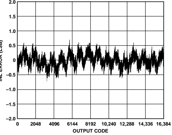
Figure 15. AD9649-80 INL Error with f_{IN} = 9.7 MHz
