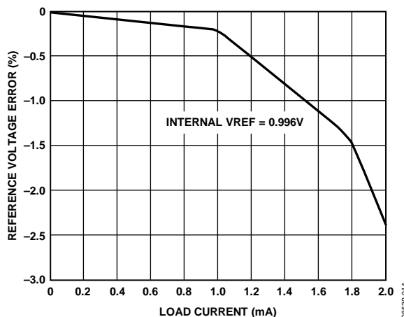
Figure 44. VREF Accuracy vs. Load Current
