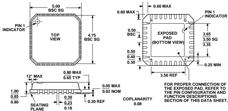
Figure 56. 32-Lead Lead Frame Chip Scale Package [LFCSP_VQ] 5 mm × 5 mm Body, Very Thin Quad (CP-32-4) Dimensions shown in millimeters
