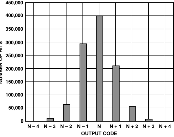
Figure 14. AD9649-80 Grounded Input Histogram
