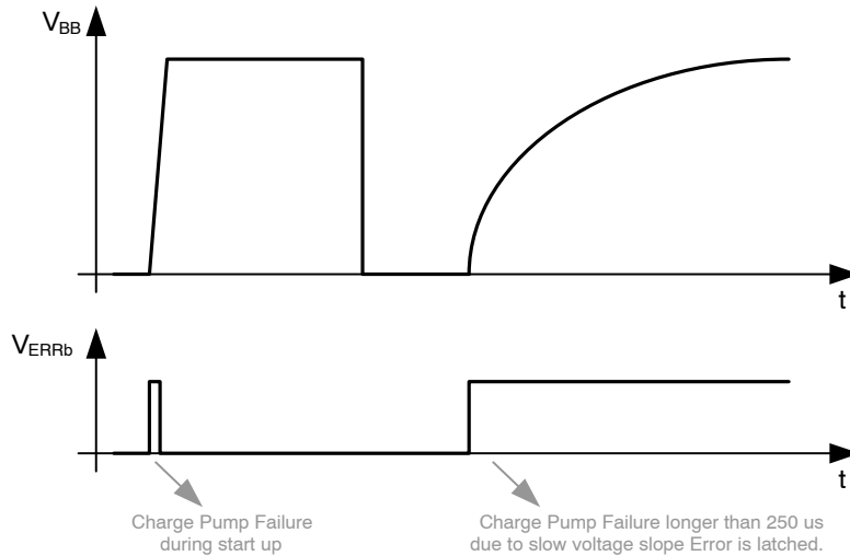
Figure 22. Charge Pump Failure
