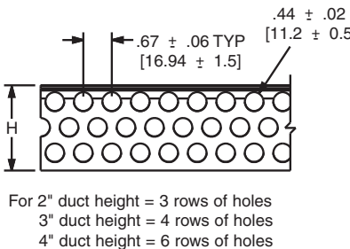
Mounting Hole Dimensions For .5", .75", 1", and 1.5" wide duct.
