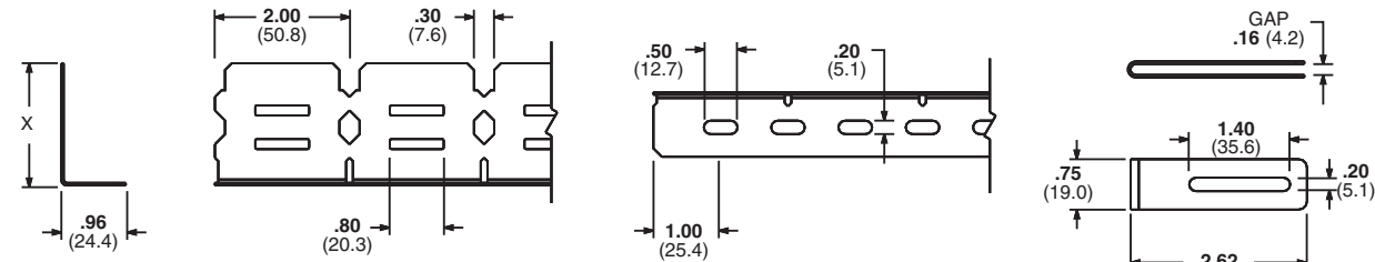
Bottom view. Bonding clip (for use with wiring duct). All dimension shown in inches (mm).
