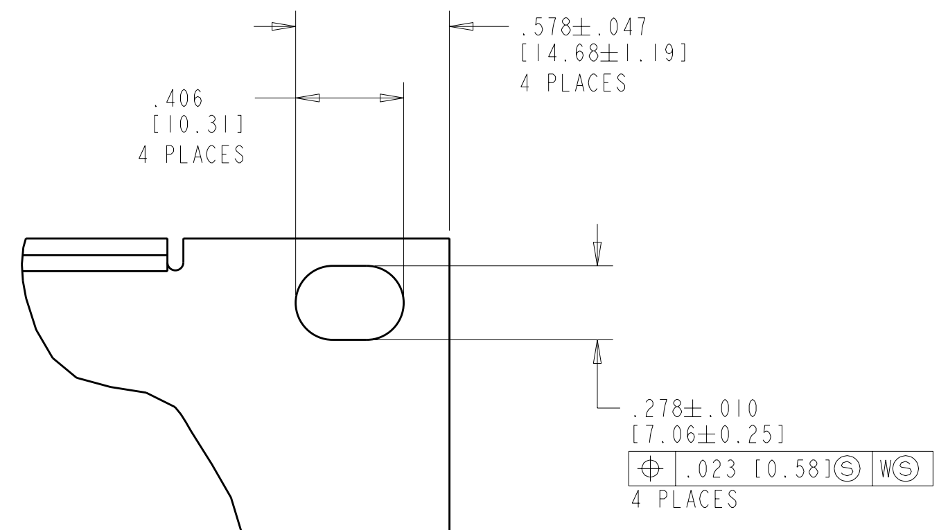
DETAIL A 556965-1 & -2 ONLY SCALE 2:1
