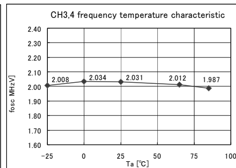
Fig.4 Frequency CH3,4—Temp
