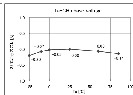
Fig.5-3 CH5 Base voltage—Temp
