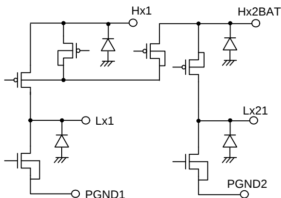
Fig.35 PIN equivalent circuit
