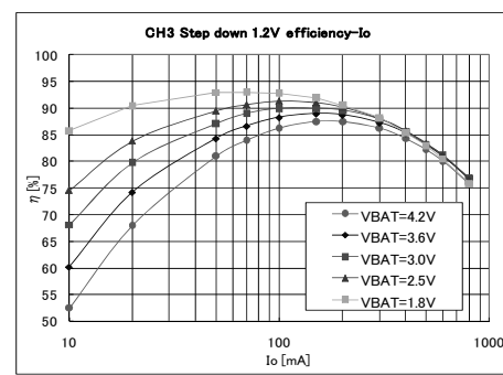
Fig.8 CH3 1.2V step-down efficiency—I o
