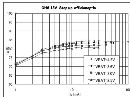
Fig.11 CH6 13V boost efficiency—I o
