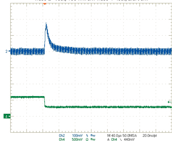
Step Load Transient Response (Vin=12V, Vout=2.5V, Clod=0, Iout=3A to 1.5A) Trace 2=Vout, 100 mV/div. Trace 4=Iout, 2.5A/div.
