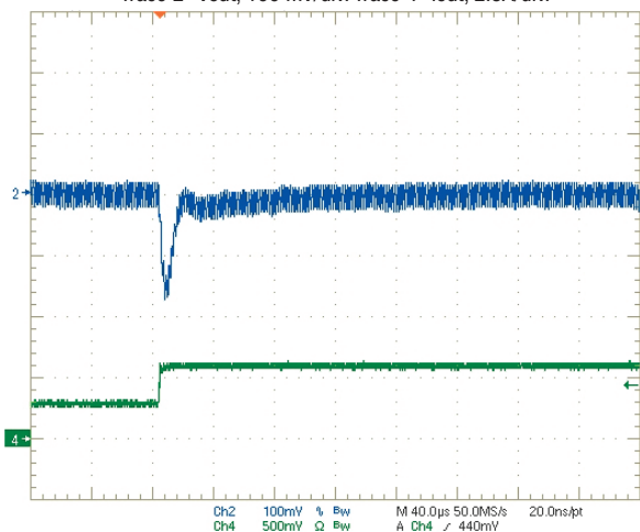
Step Load Transient Response (Vin=12V, Vout=2.5V, Clod=0, Iout=1.5A to 3A) Trace 2=Vout, 100 mV/div. Trace 4=Iout, 2.5A/div.
